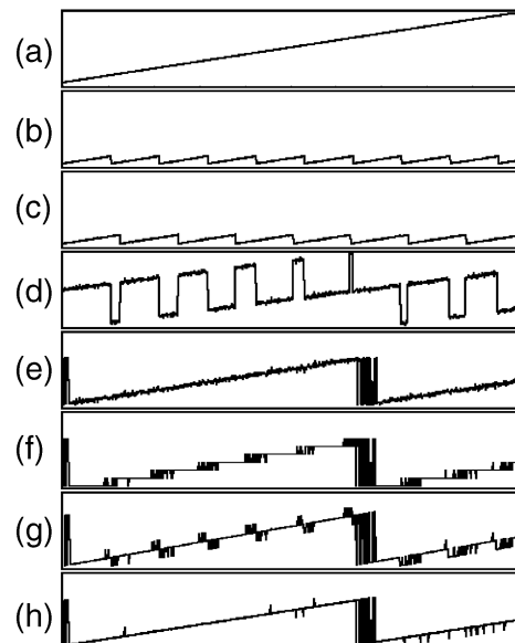
Fig. 1. Simulation of two-wavelength phase imaging. See text for details.
